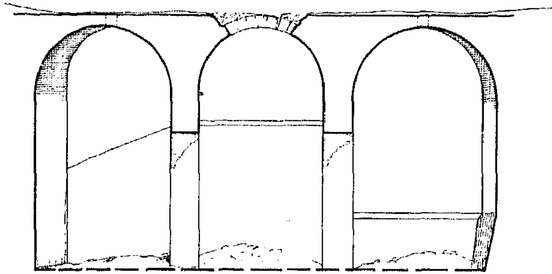
Section C-C
